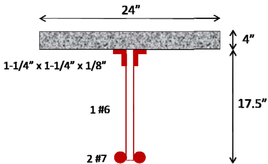
Figure 41 – Specimen No.1 Section
