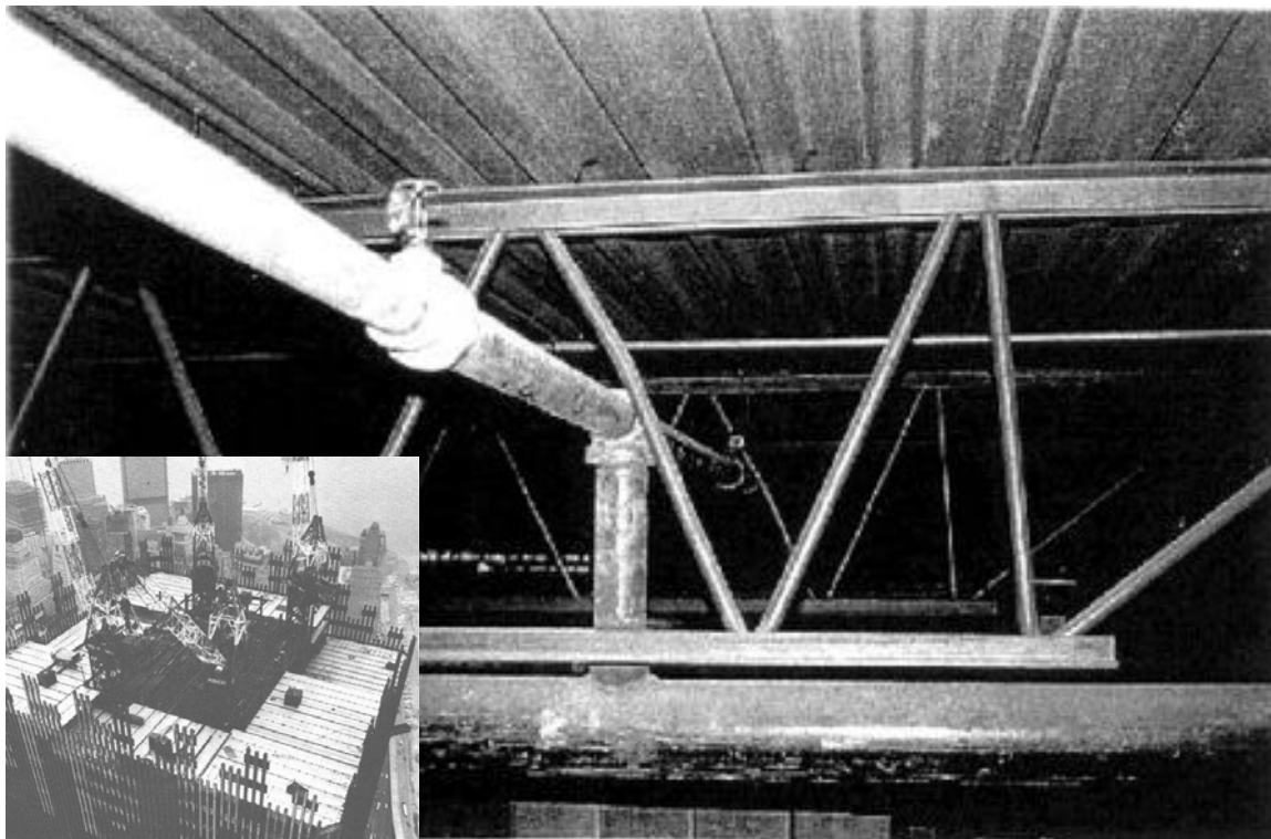
Figure 8 – Open-Web Steel Joist: WTC, New York, 1960
