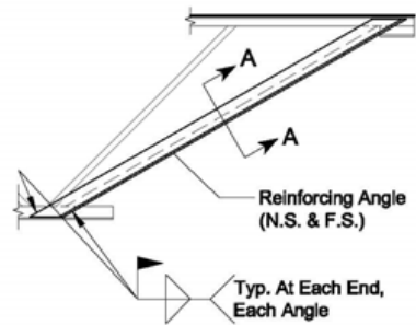
Figure 30 – End Diagonal Reinforcing (Fisher, 2004)
